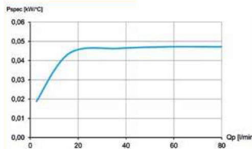
Specific cooling performance
