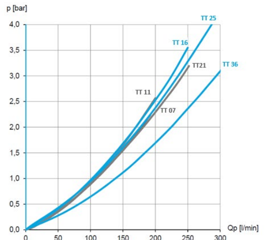
Pressure drop at 30°C
